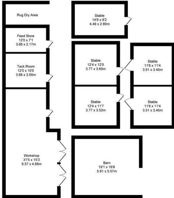
Outbuildings Approx. Floor Area 2289 Sq.Ft (212.7 Sq.M.)
